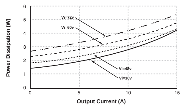
Power Dissipation vs. Output Current for 2.5V/15A PKM4319PI
