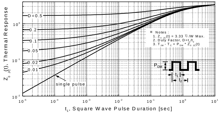
Figure 11-2. Transient Thermal Response Curve for IRFS630B
