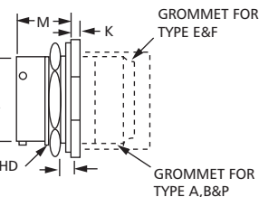
CRIMP KPSE07/MS3124
