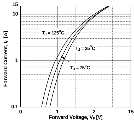
Figure 19. Forward Characteristist
