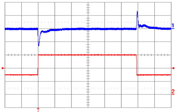
Fig. 21: Output voltage response to load current step-change (7.5 A – 15 A – 7.5 A) at V_{in} = 24\text{ V} . Top trace: output voltage (100 mV/div). Bottom trace: load current (5 A/div.). Current slew rate: 5 A/ \mu\text{s} . C_o = 450\text{ }\mu\text{F} tantalum + 1 \mu\text{F} ceramic. Time scale: 0.2 ms/div.
