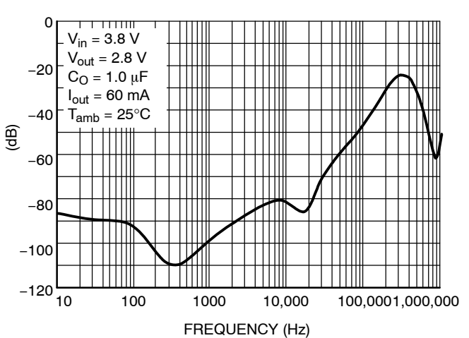
Figure 32. Ripple Rejection versus Frequency without Bypass Capacitor
