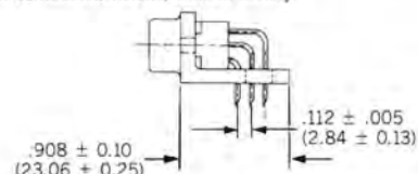
DDP-50S CONTACT ARRANGEMENT
