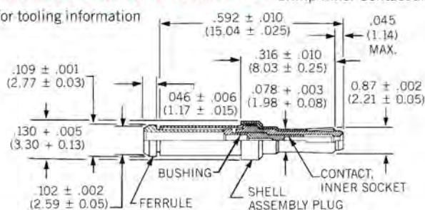
PLUG: DDMA110335 — RG196A/U and RG179B/U cable
