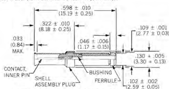
RECEPTACLE: DDMA110336 — RG196A/U and RG173B/U cable
