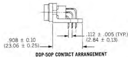
DDP-50P CONTACT ARRANGEMENT
