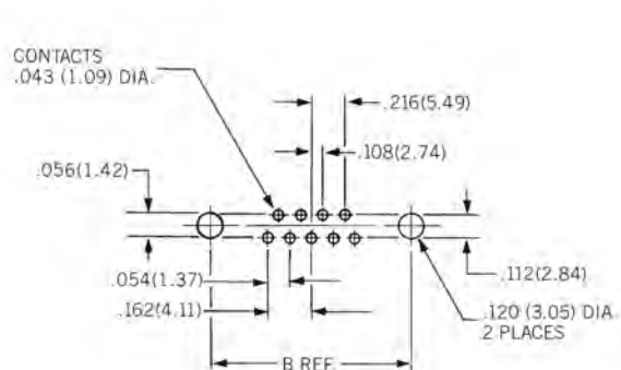
9 POSITION PCB HOLE PATTERN
