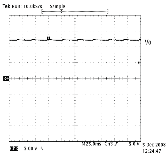
Figure 15. Typical Output Voltage in Burst Operation (TP15)
