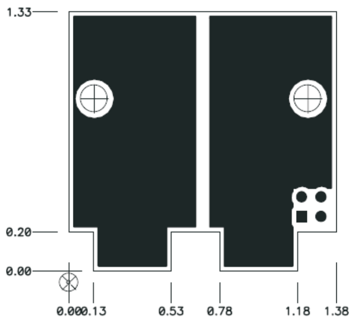
Figure 23. Top Copper
