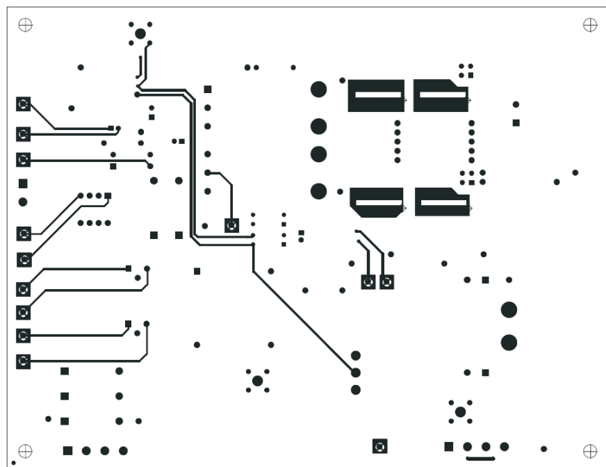
Figure 19. Top Copper
