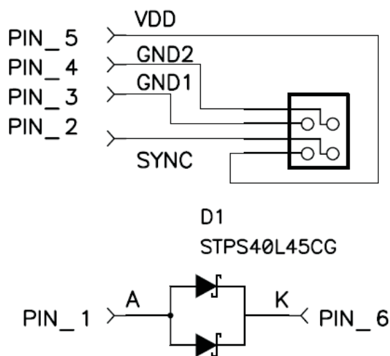
Figure 26. Schematics
