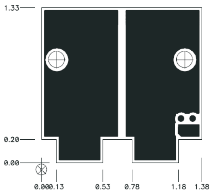
Figure 25. Bottom Copper
