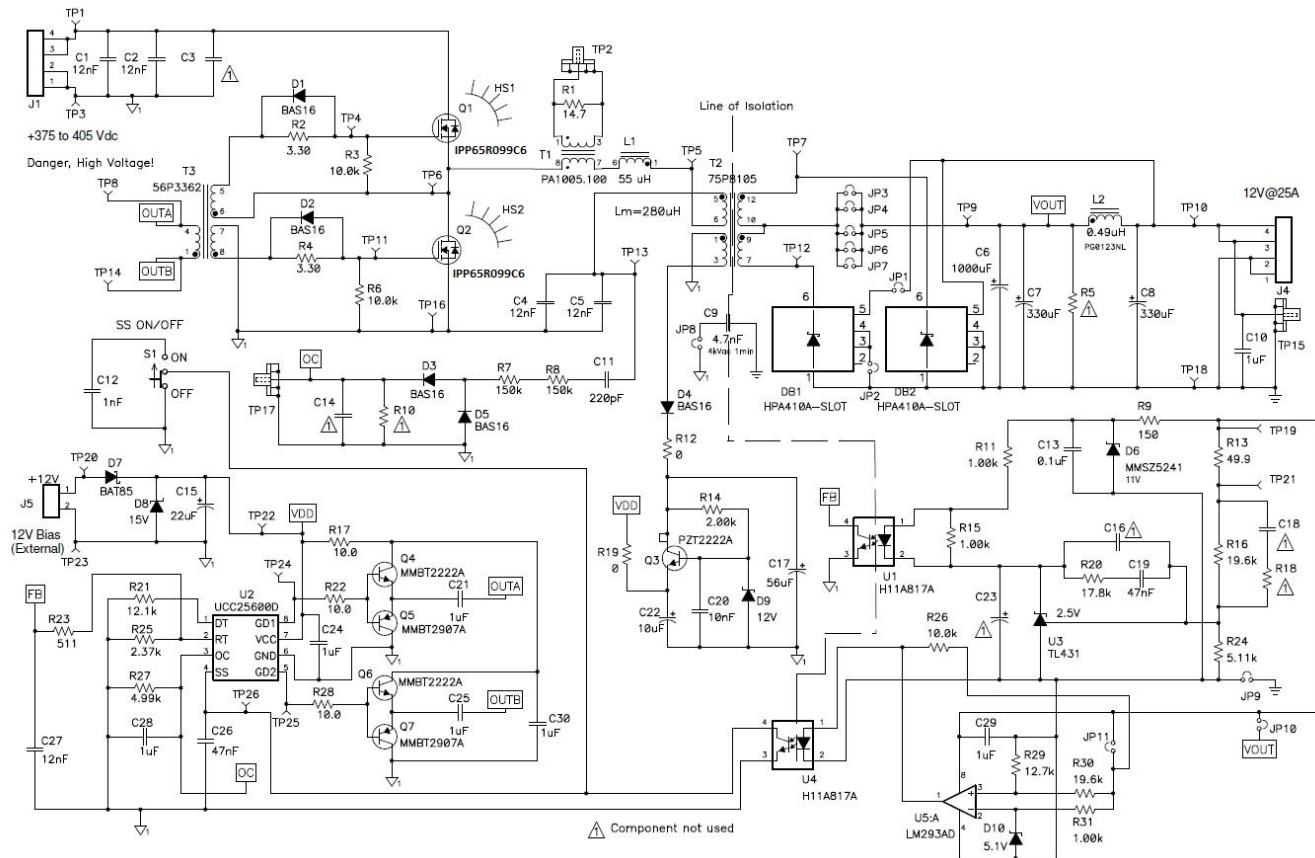
Figure 1. UCC25600EVM Schematic
