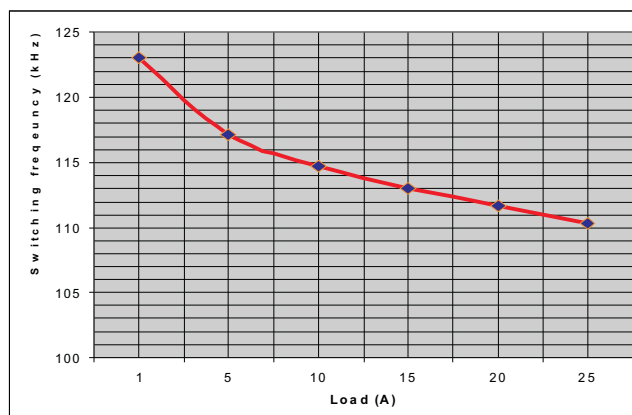
Figure 17. Switching Frequency Variation with Respect to Load (TP24)
