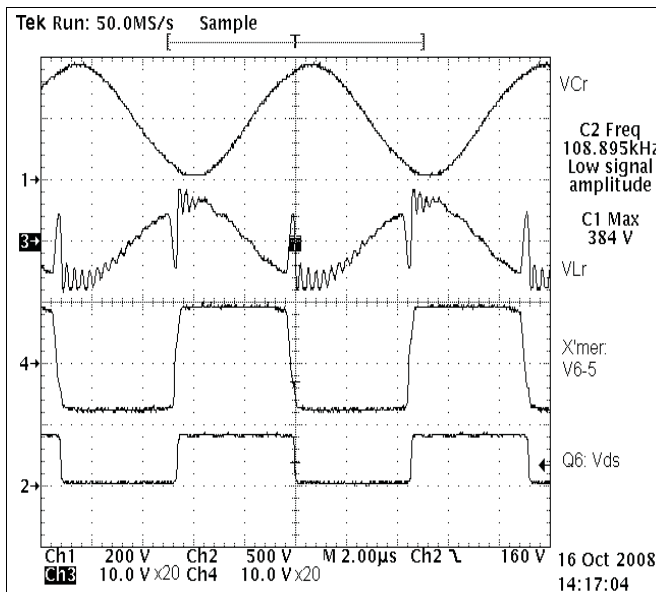
Figure 12. Typical Voltage of the Resonant Circuit
