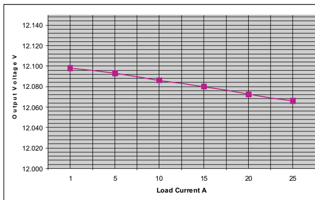
Figure 5. Load Regulation, V_{IN} = 390 V DC
