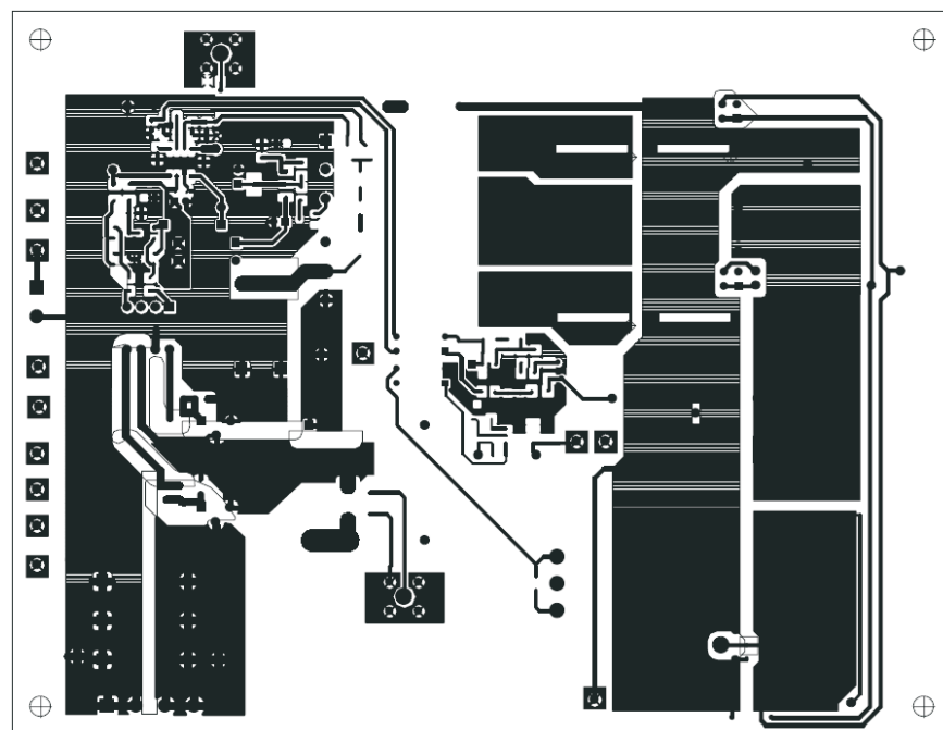
Figure 21. Bottom Copper
