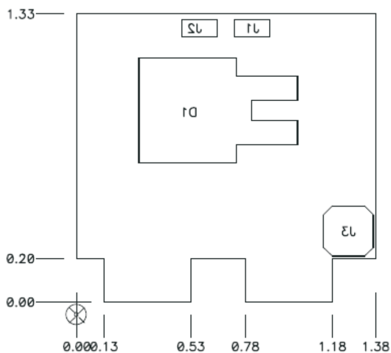
Figure 24. Bottom Assemblies
