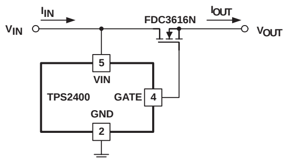
Figure 1. Application Diagram
