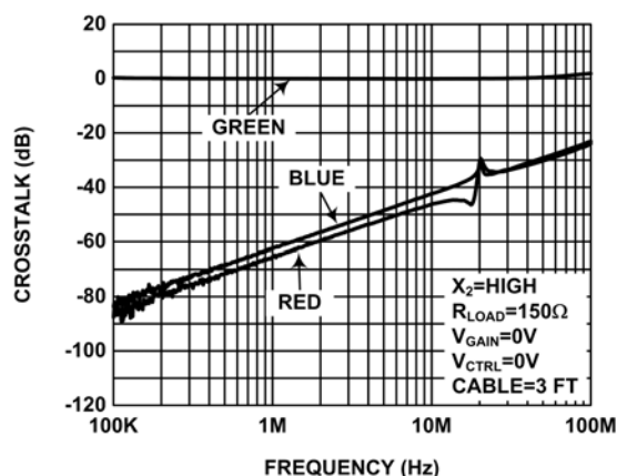
FIGURE 17. GREEN CROSSTALK
