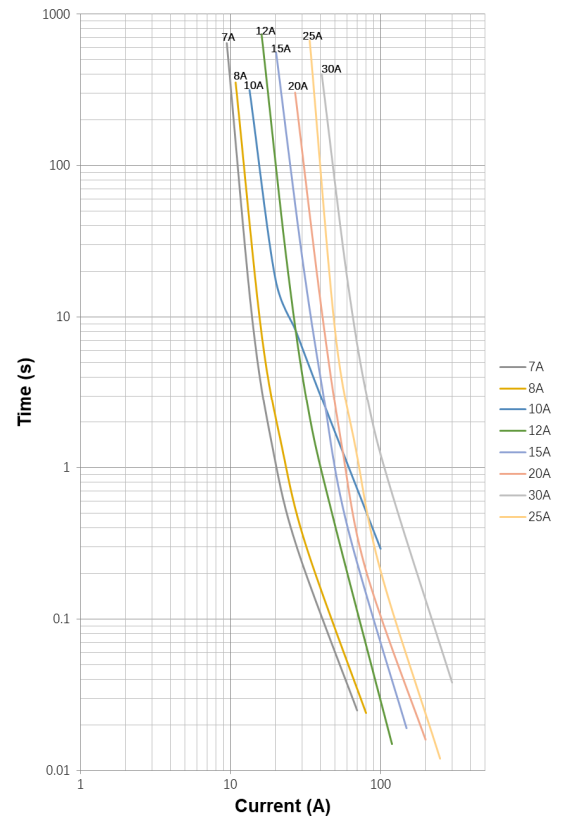
Time-current curves (7 A - 30 A)
