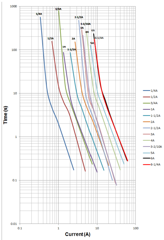
Time-current curves (1/4 A - 6 1/4 A)
