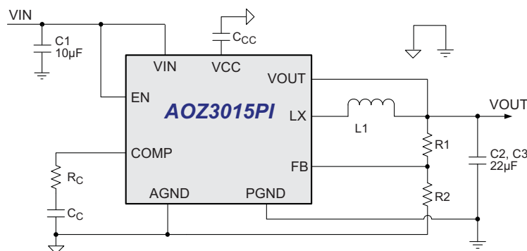
Figure 1. 3 A Synchronous Buck Regulator, F_s = 500 \text{ kHz}
