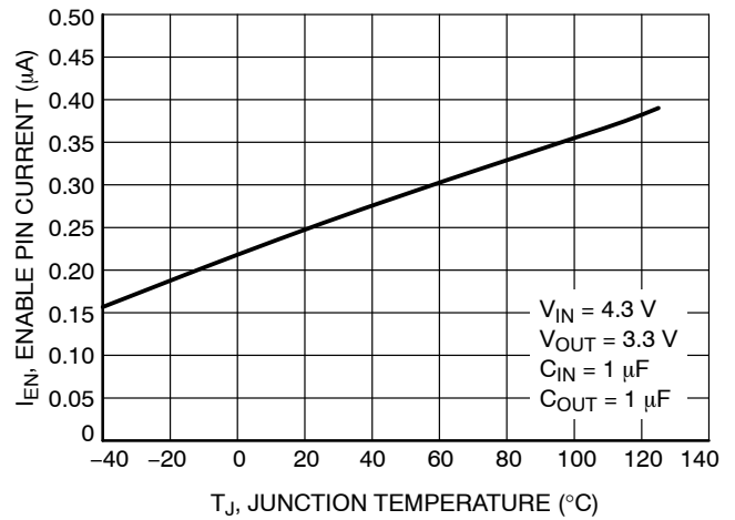
Figure 28. Enable Current Temperature
