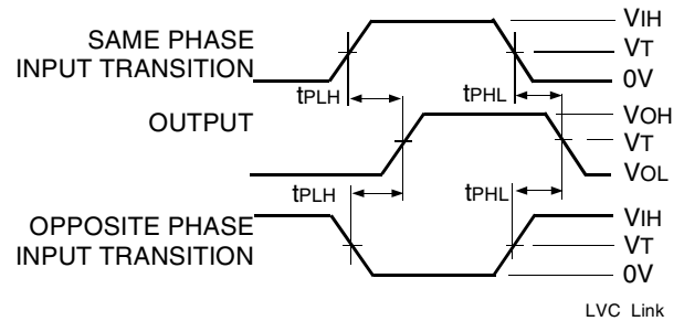
Propagation Delay
