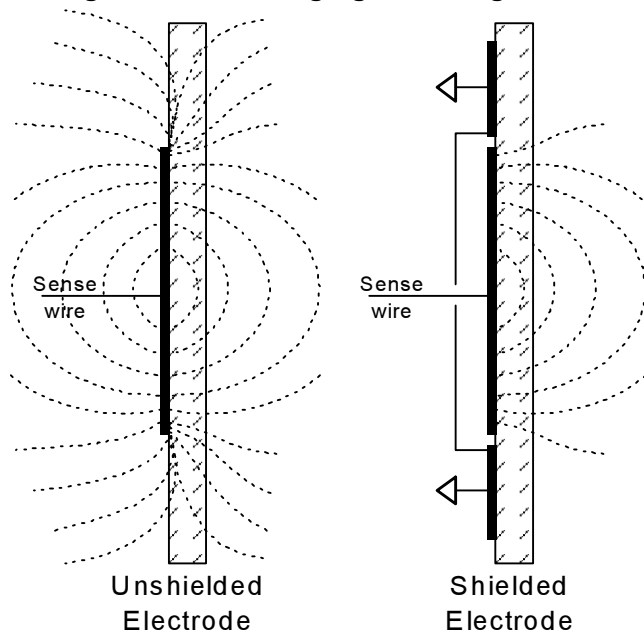
Figure 1-4 Shielding Against Fringe Fields
