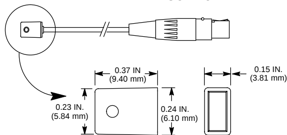
SM93/WL93 MICROPHONE
