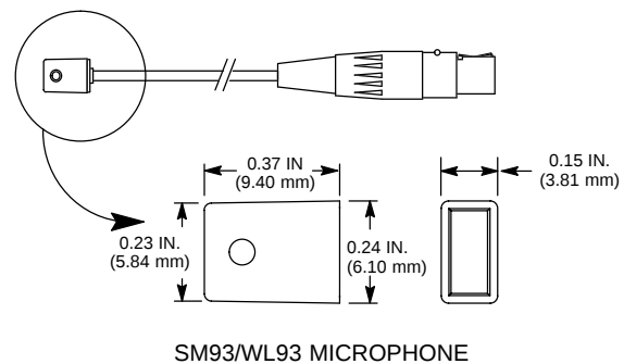
OVERALL DIMENSIONS FIGURE 5
