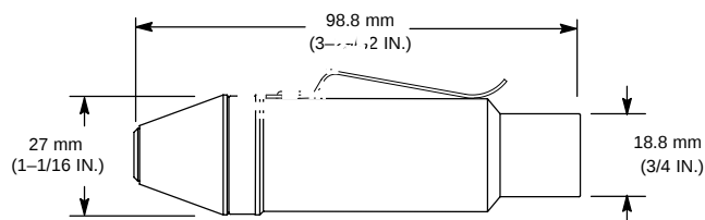
SM93 PREAMPLIFIER
