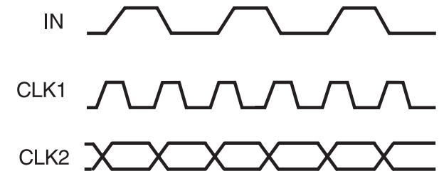
Input and Output Clock Waveforms with CLK1 Connected to FBIN
