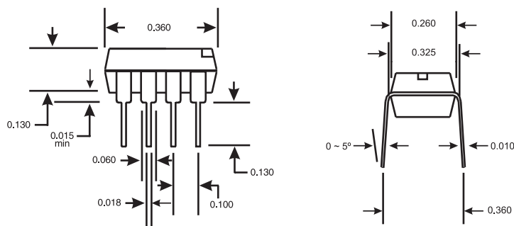
8-Pin DIP PACKAGE
