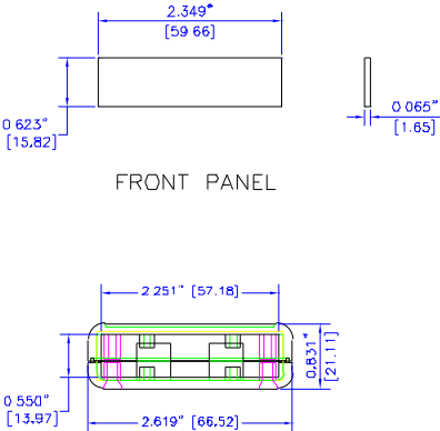
ASSEMBLED VIEW
