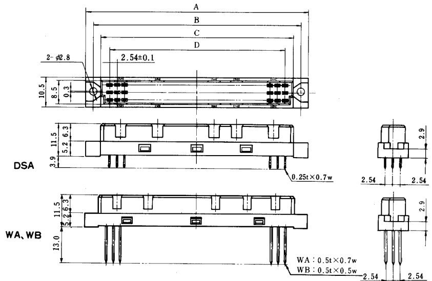
PCN10*S-2.54DSA
