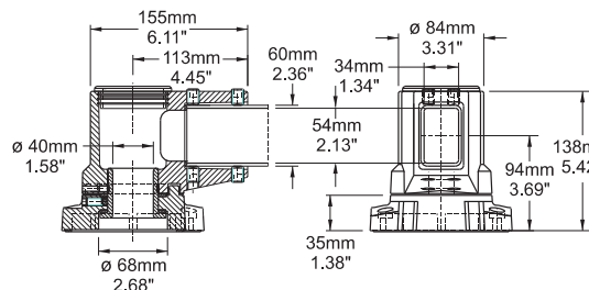
Front Section Socket Joint
