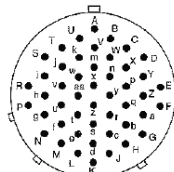
Shell Size 24 48
