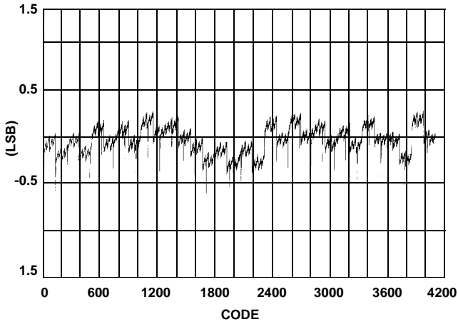
FIGURE 6. TYPICAL INL
