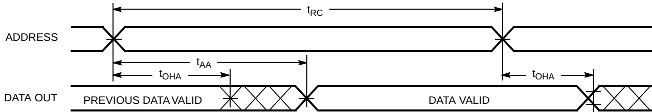
Read Cycle No. 2 (Either Port \overline{\text{CE}}/\overline{\text{OE}} Access) [24, 27, 28]
