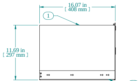
SIDE VIEW WITHOUT SHROUD
