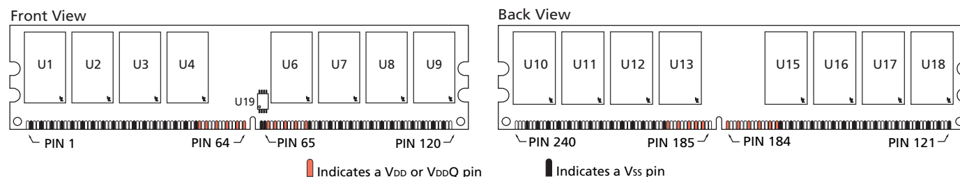
Figure 2: Pin Locations
