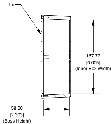
Top View Looking Inside Box
