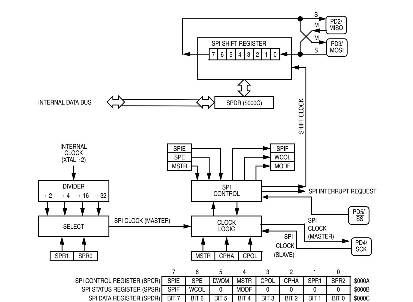
Figure 10-2. Serial Peripheral Interface Block Diagram
