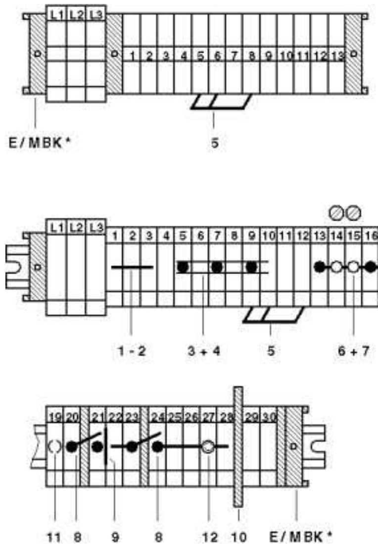
Circuit diagram
