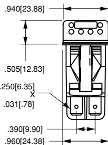
8 TERMINAL BASE W/BARRIERS
