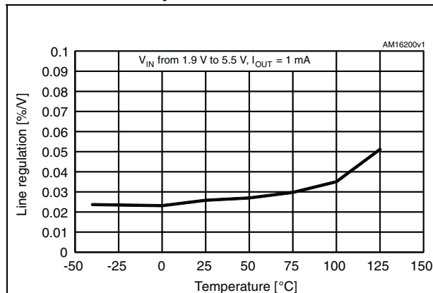
Figure 10. Line regulation vs. temp. for adjustable version
