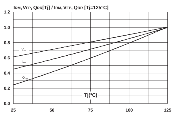
Fig. 10: Relative variations of dynamic parameters versus junction temperature.
