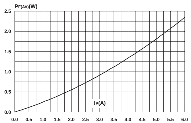
Fig. 1-2: Power dissipation versus peak forward current (triangular waveform, \delta = 0.45 ) (modulation diode).
