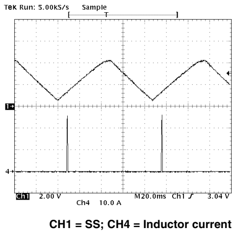
Figure 8. Hiccup Mode
