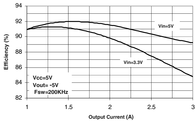
Figure 33. Efficiency vs. Output Current
