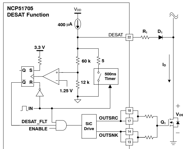
Figure 39. NCP51705 DESAT Function
