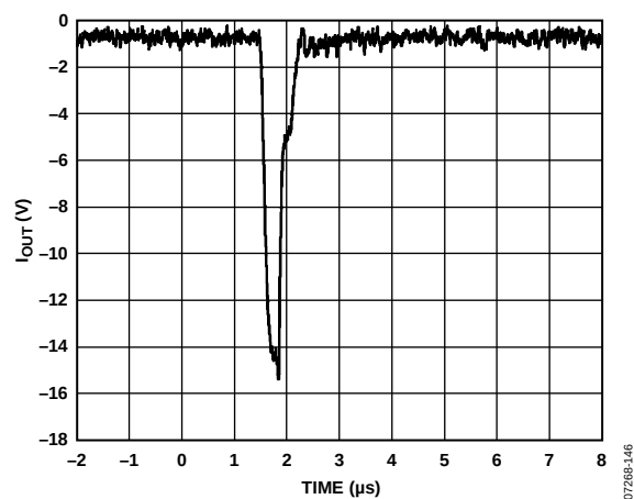
Figure 46. Output Current vs. Time on Output Enable
