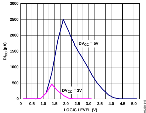
Figure 48. D_{I_{CC}} vs. Logic Input Voltage
