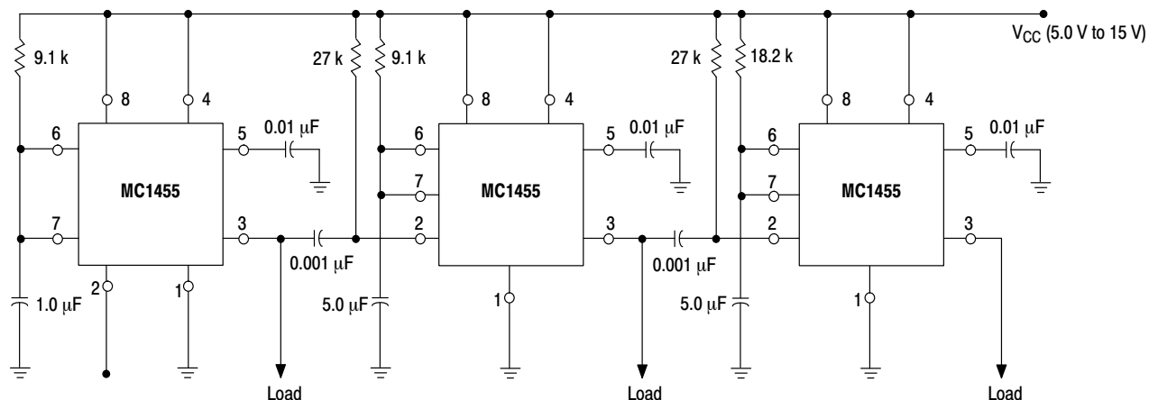
Figure 26. Sequential Timer
