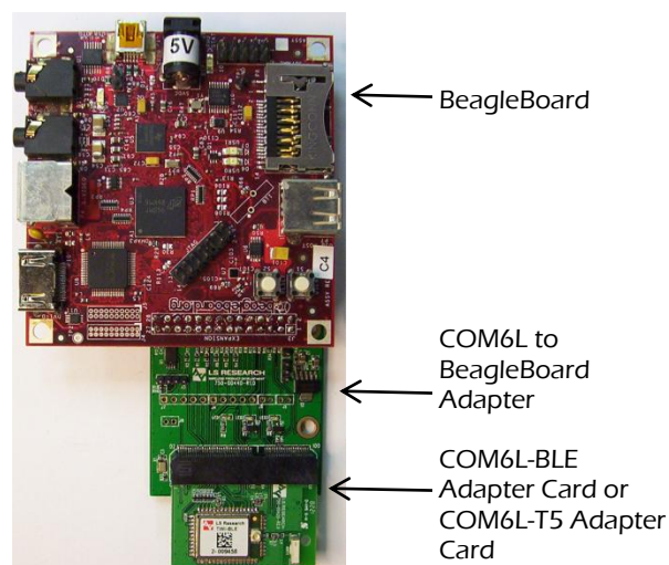
COM6L to BeagleBoard Adapter interfacing the BeagleBoard to LSR's COM6L-BLE Adapter Card or COM6L-T5 Adapter Card
