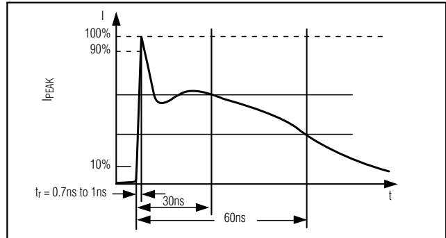
Figure 6b. IEC 1000-4-2 ESD Generator Current Waveform
