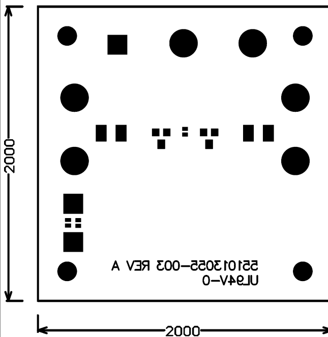
Figure 4-8. Bottom Soldermask
