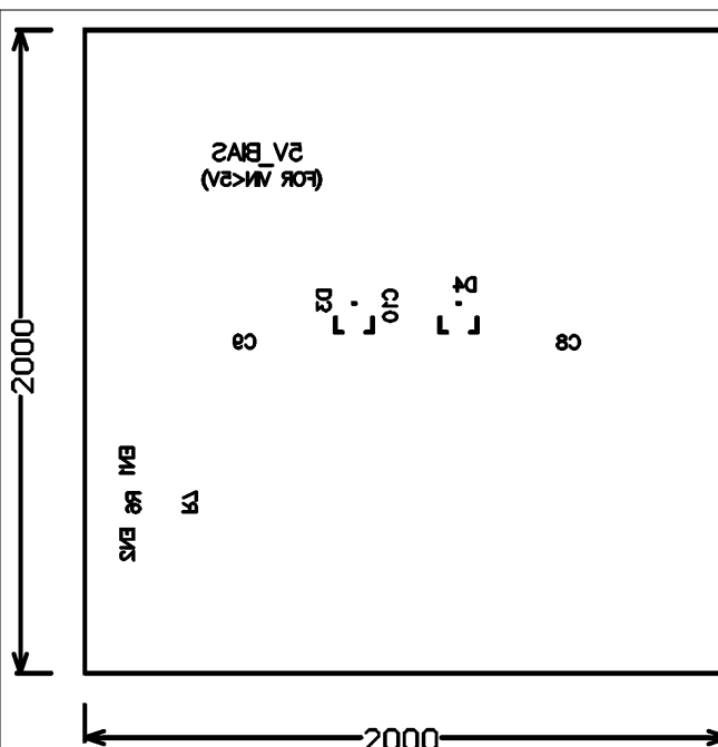
Figure 4-6. Bottom Silkscreen
