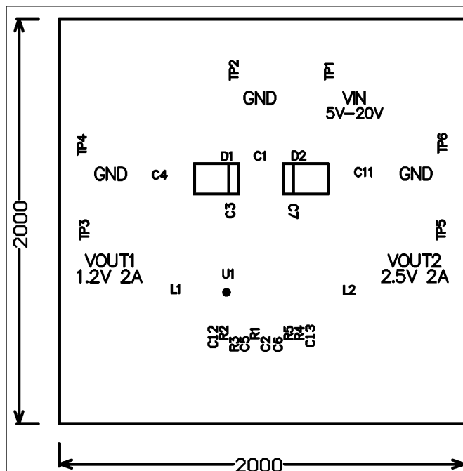
Figure 4-5. Top Silkscreen
