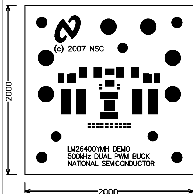
Figure 4-5. Top Silkscreen
