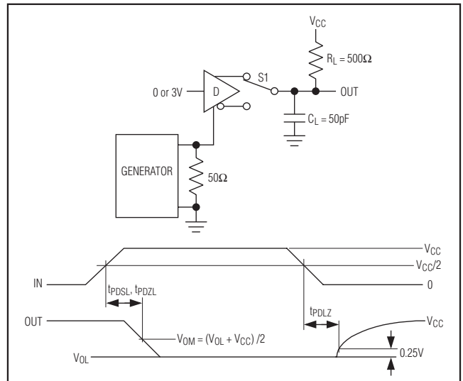
Figure 4. Driver Enable and Disable Times ( t_{PDSL} , t_{PDLZ} , t_{PDL} , t_{PDLZ} )
