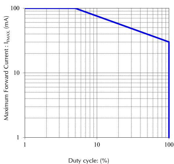
Duty Cycle vs. Max. Forward Current
