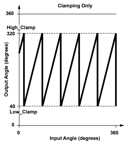
Figure 23: CE = 0, ROE = 1. Applied gain = 4x. LOW_CLAMP = 10 (≈40°), HIGH_CLAMP = 10 (≈320°)
