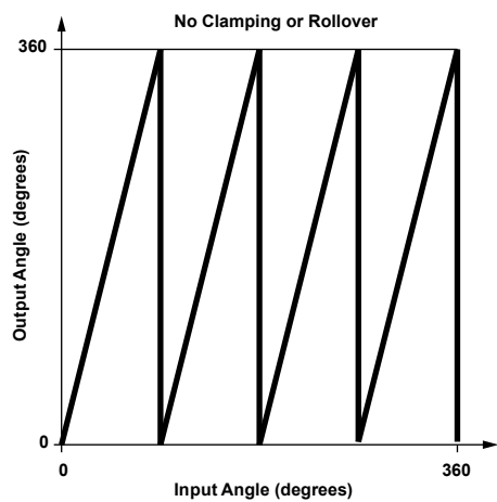
Figure 21: CE = 0, ROE = 0. Applied gain = 4x.
