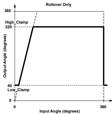
Figure 22: CE = 1, ROE = 0. Applied gain = 4x. LOW_CLAMP = 10 (≈40°), HIGH_CLAMP = 10 (≈320°)
