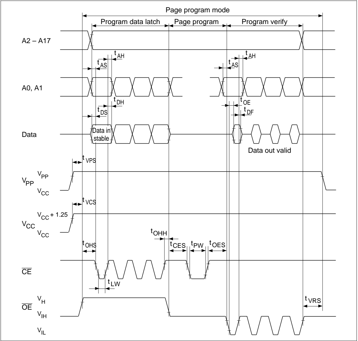
Fast High-Reliability Page Programming Timing Waveform
