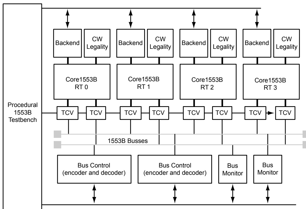
Figure 6-1 • Verification Testbench
