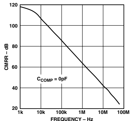
TPC 13. Common-Mode Rejection Ratio vs. Frequency
