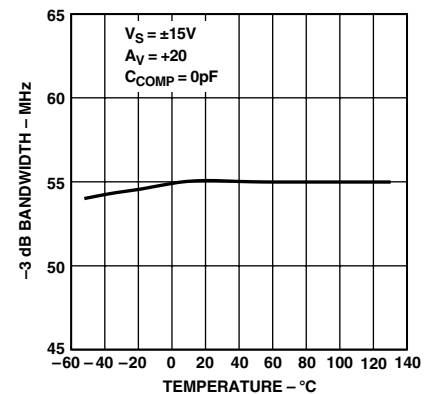
TPC 9. -3 dB Bandwidth vs. Temperature
