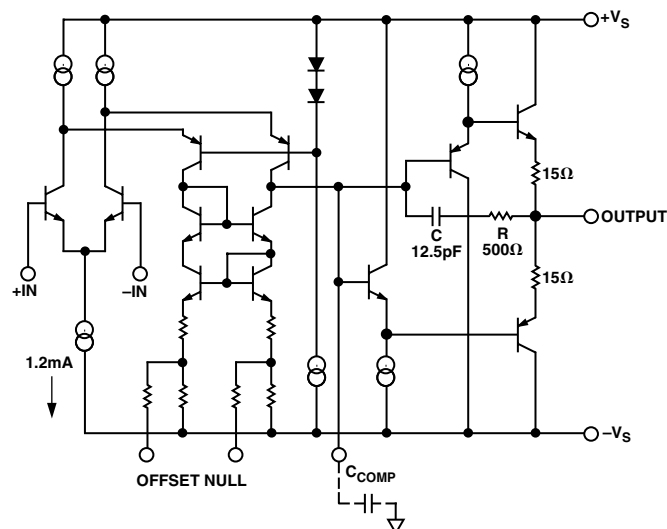
Figure 5. Simplified Schematic
