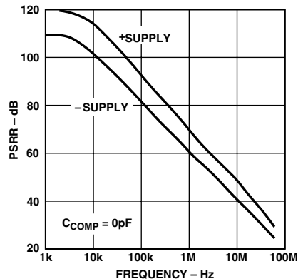
TPC 12. Power Supply Rejection Ratio (PSRR) vs. Frequency
