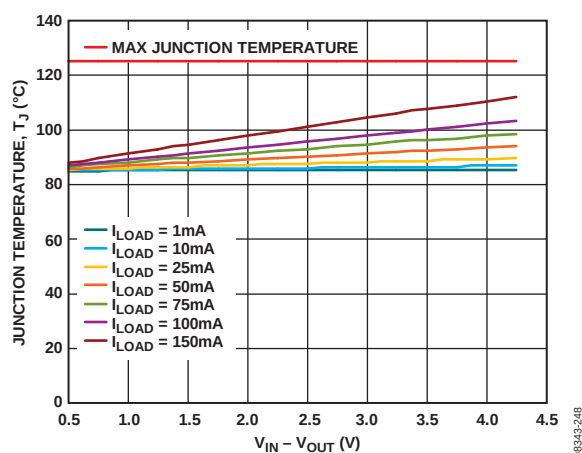
Figure 39. TSOT, 100 mm² of PCB Copper, Board Temperature = 85°C
