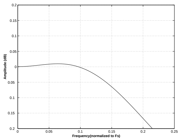
Figure 43. Quad-Speed (fast) Passband Ripple
