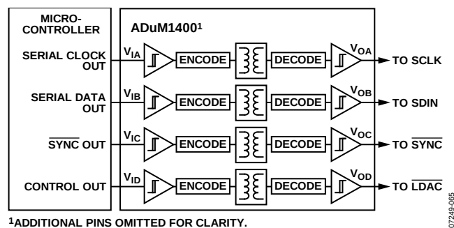
Figure 30. Isolated Interface
