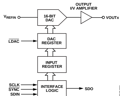
Figure 27. Simplified Serial Interface of Input Loading Circuitry for One DAC Channel
