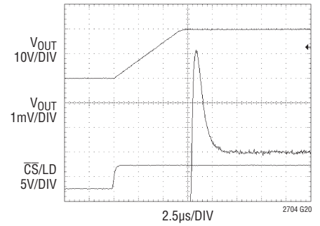
Settling ±10V
