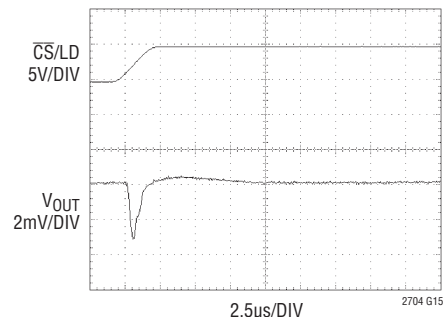
Midscale Glitch
