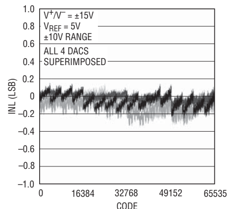
LTC2704-16 Integral Nonlinearity (INL)
