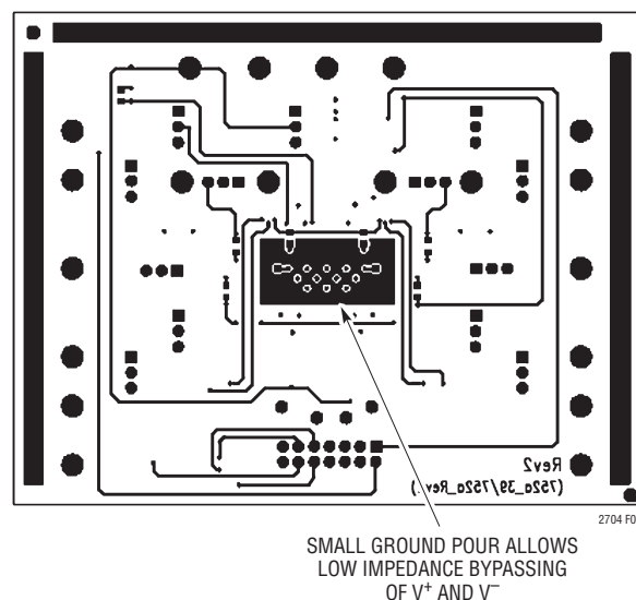
Figure 6. DC752A Routing, Bypass
