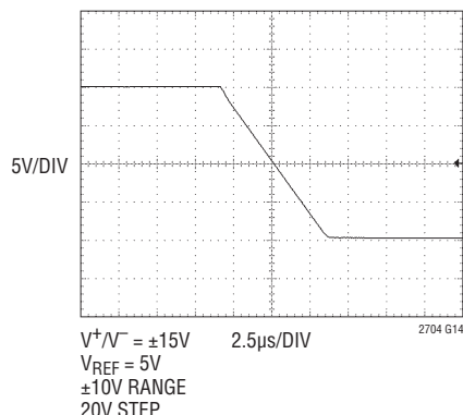
Negative Slew
