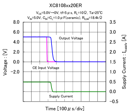
(21) turn-off Delay vs. Fall Time ( C_L=1.0\mu F )
