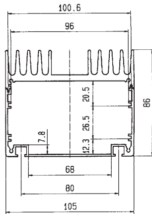
Enclosure Profiles
